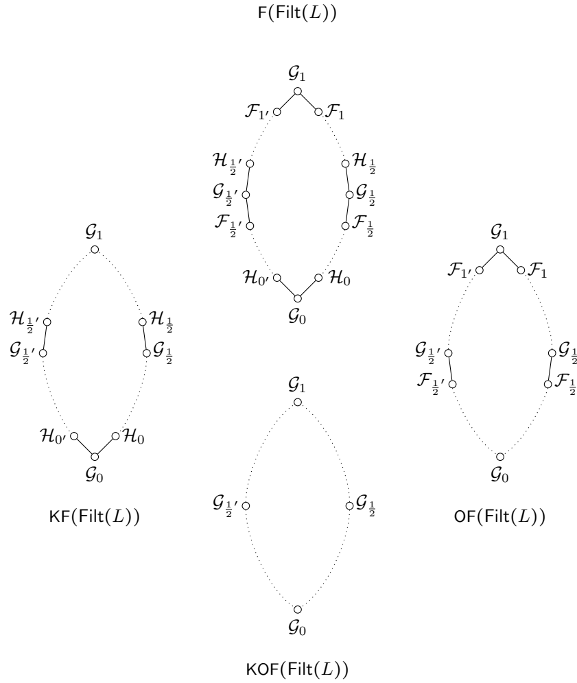
FIGURE 5. Sets of filters in \text{Filt}(L) ordered by inclusion
